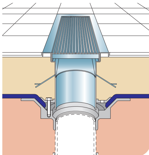
RE channel and SS3135A5 grating with D1004 non-trapped body and C.D10LW membrane clamping collar.
