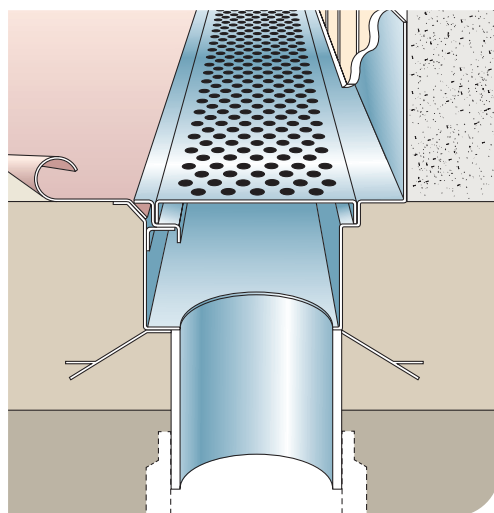
SVFT channel (SVF with optional tile upstand) and SS40135A1 grating. wadetech@alumascwms.co.uk
