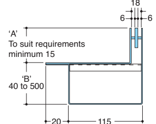
Spec. Code: HSCE Designed for use against a wall. With non-removable toe bar. 6mm slot width suitable for use in barefoot areas.
