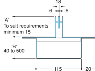
Spec. Code: HSC With non-removable toe bar. 6mm slot width suitable for use in barefoot areas.
