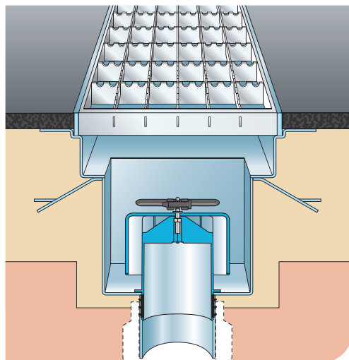
NEF channel and SS7300A5 grating with Q14 style dropped sump and U1704 removable bell trap.
